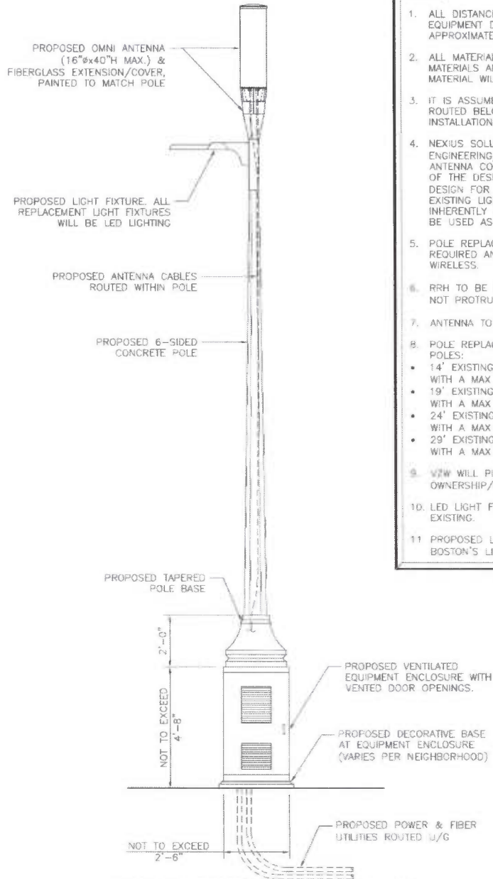
AERIATA CONCRETE LIGHT POLE W/ RRH CONCEALMENT
