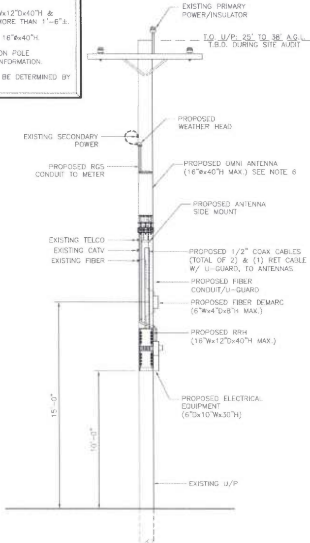
WOOD UTILITY POLE WITH ANTENNA SIDE MOUNT
