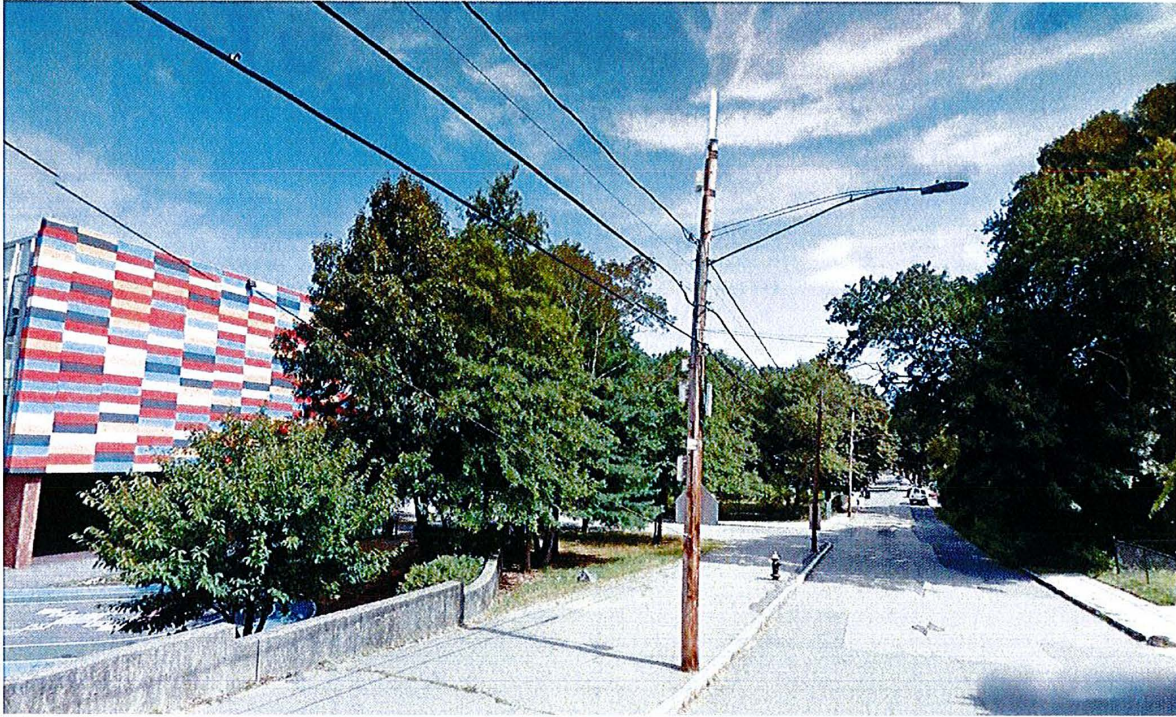
Example of wood utility pole with approved wireless facility installed (top mount)
