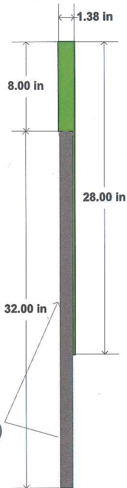
Existing Railing(Iron)
