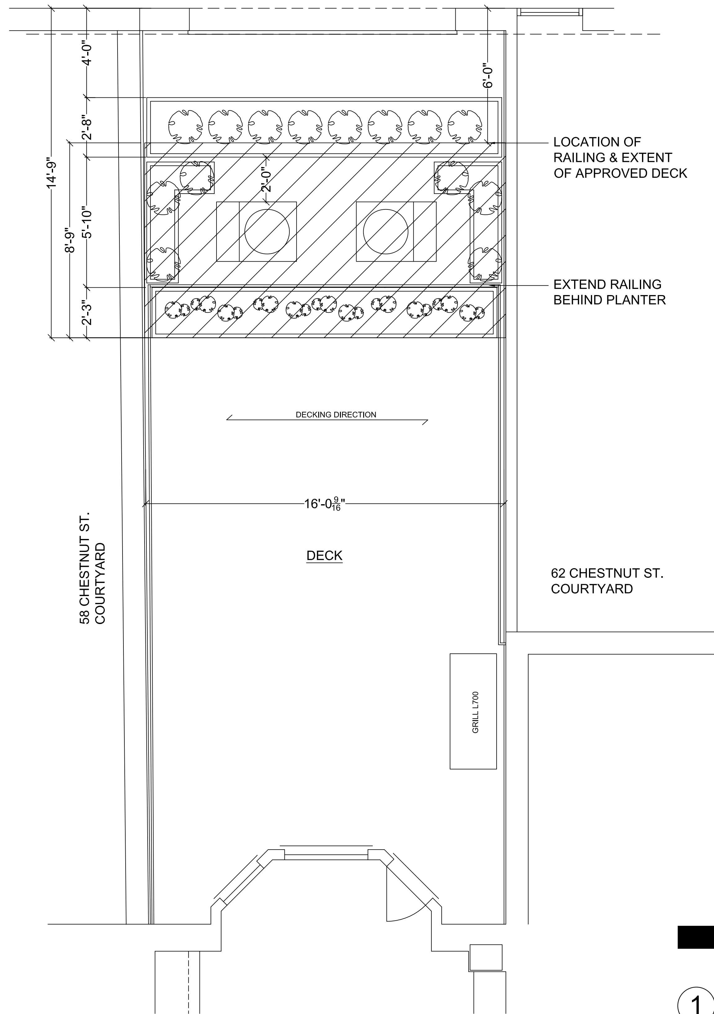
PROPOSED DECK PLAN SCALE: 3/8" = 1'-0"
