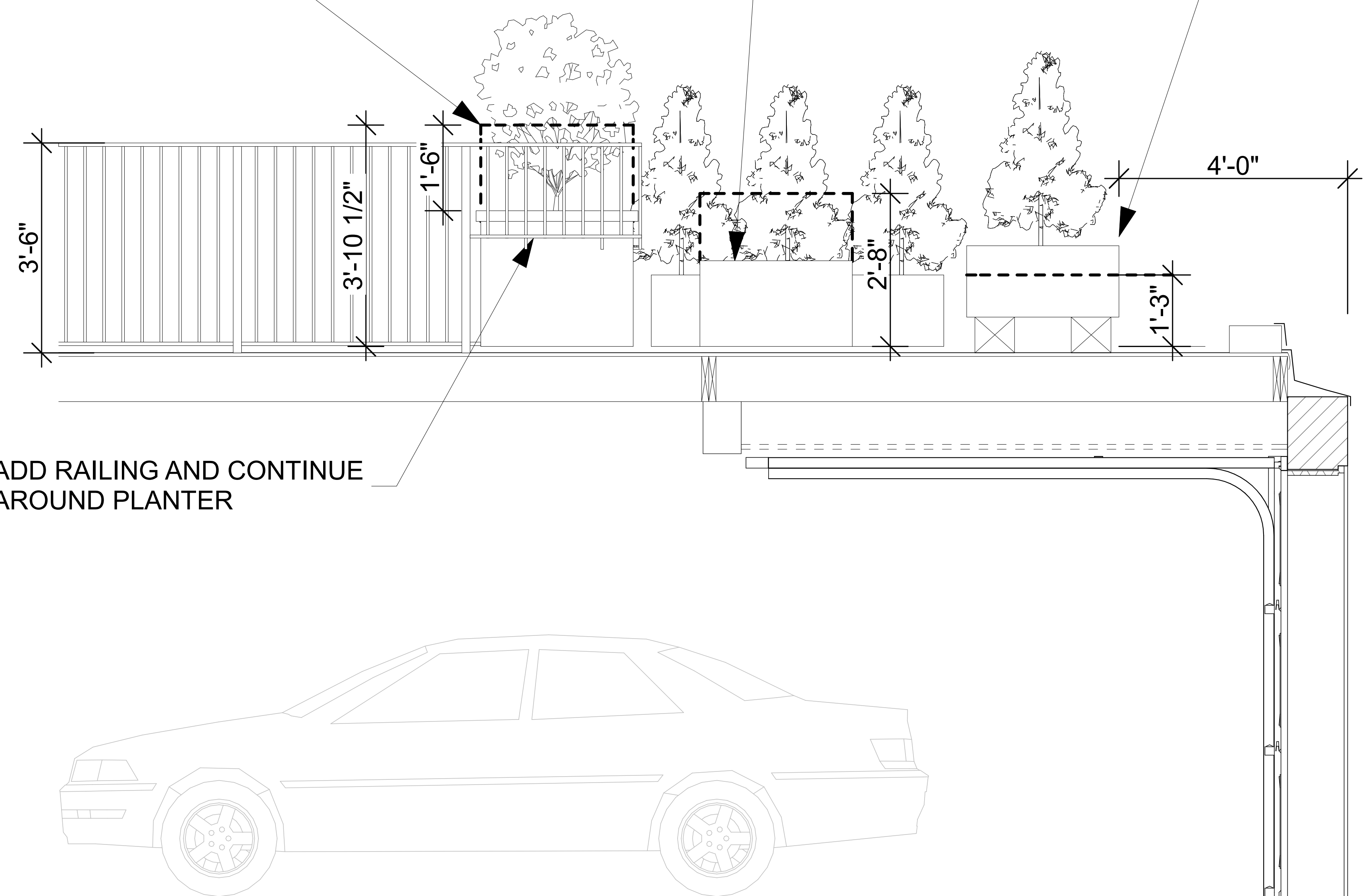
1 CROSS SECTION SCALE: 3/4" = 1'-0"
