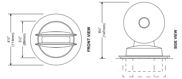
SURFACE MOUNT LED TO LIGHT THE WINDOW FRAME
