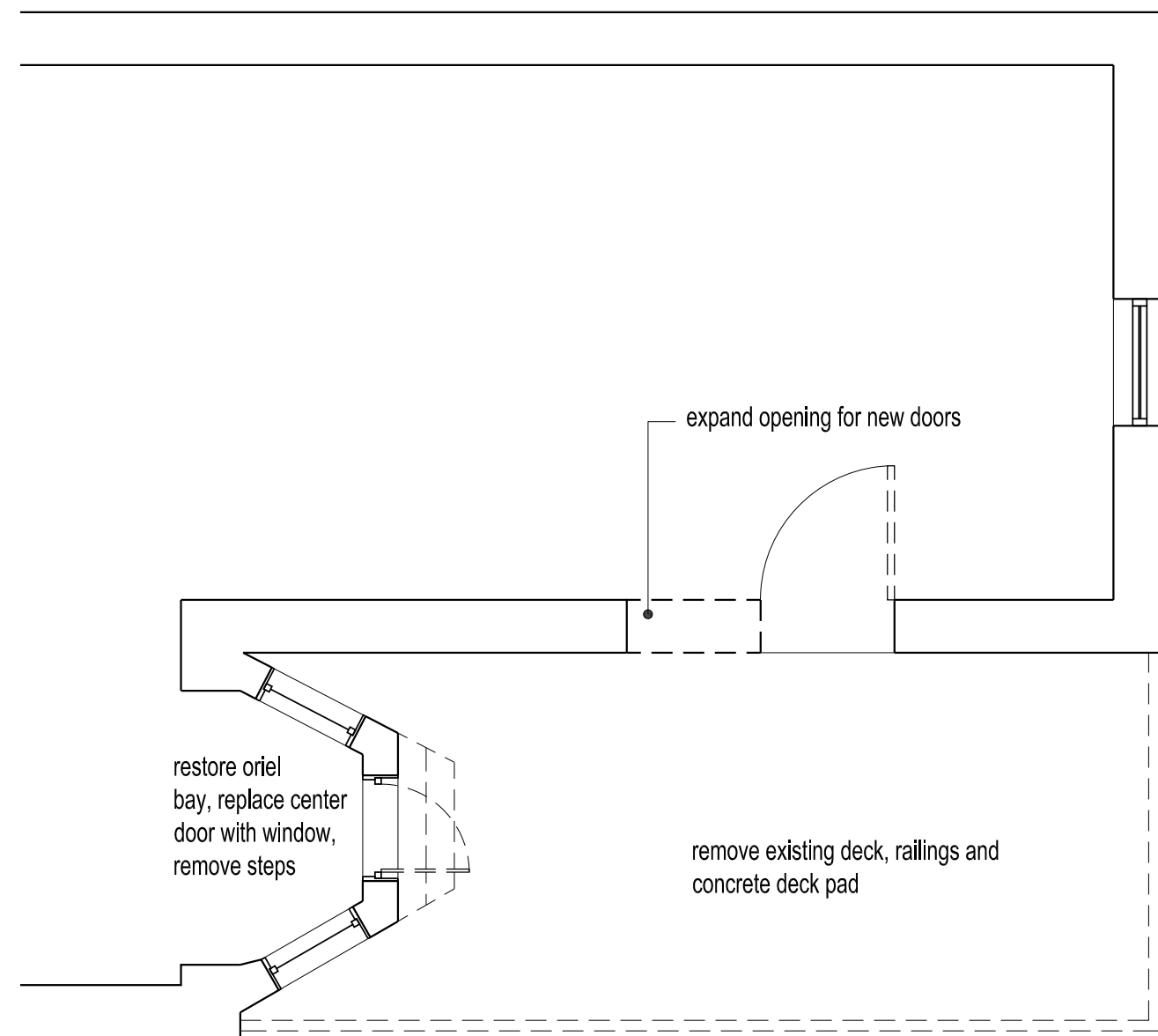
PARTIAL PLAN SHOWING DEMOLITION
