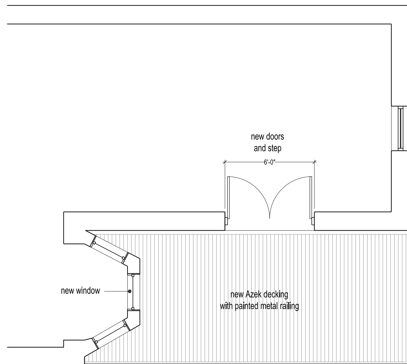
PARTIAL PLAN SHOWING PROPOSED
