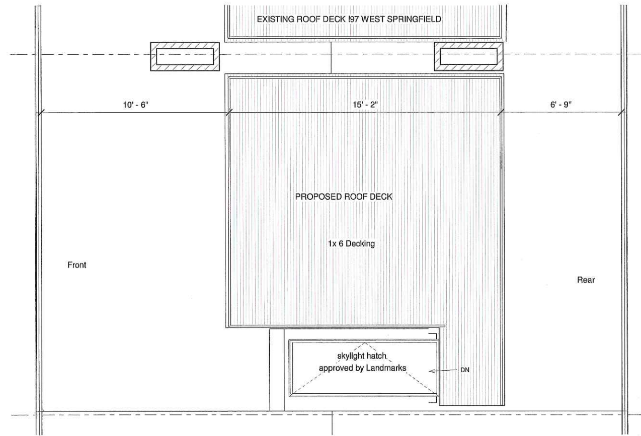
1 Roof Deck for Landmarks 3/8" = 1'-0"
