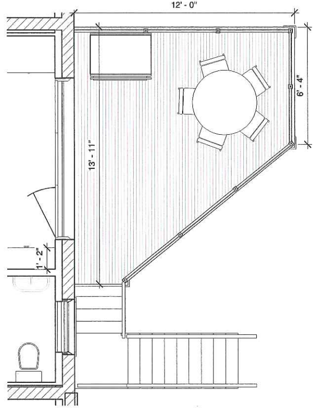
5 1st Floor Deck for Landmarks 3/8" = 1'-0"
