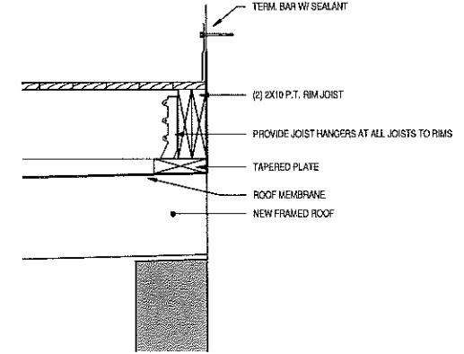
5 PROPOSED SECTION1 - Callout 1 1 1/2" = 1'-0"
