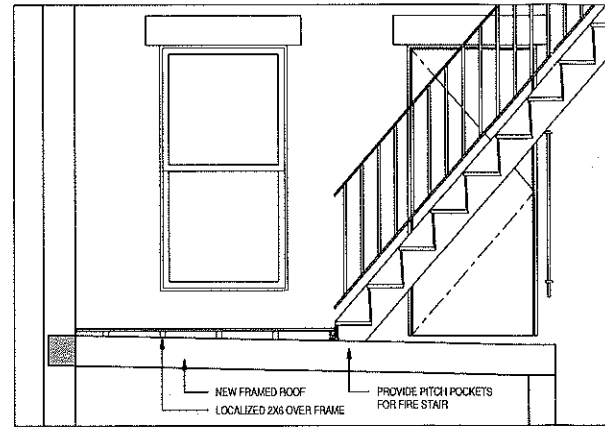
9 Section 1 1/2" = 1'-0"
