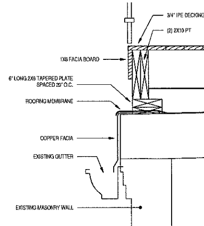
8 PROPOSED SECTION1 - Callout 2 1 1/2" = 1'-0"
