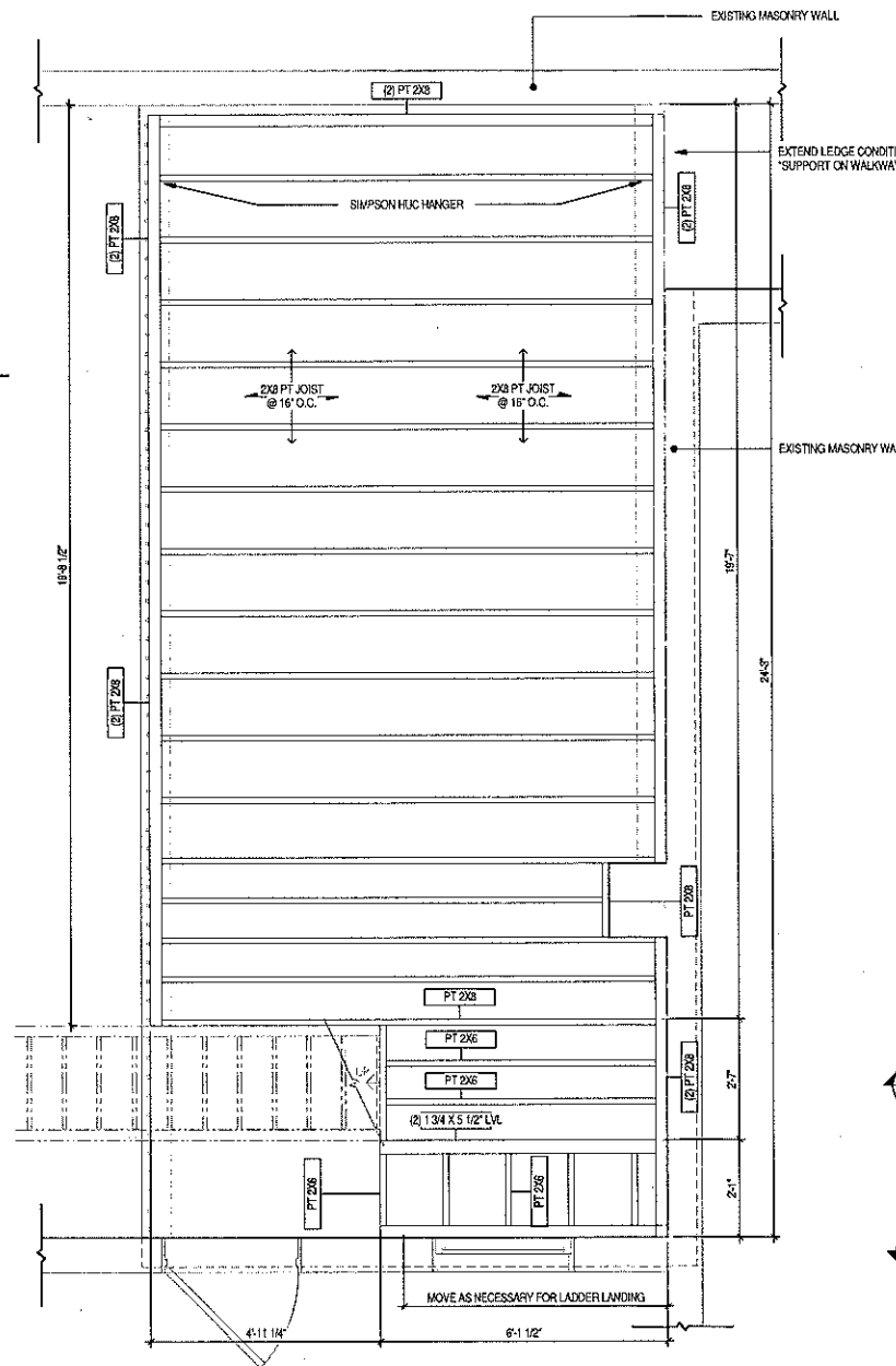
6 PROPOSED DECK FRAMING 1/2" = 1'-0"
