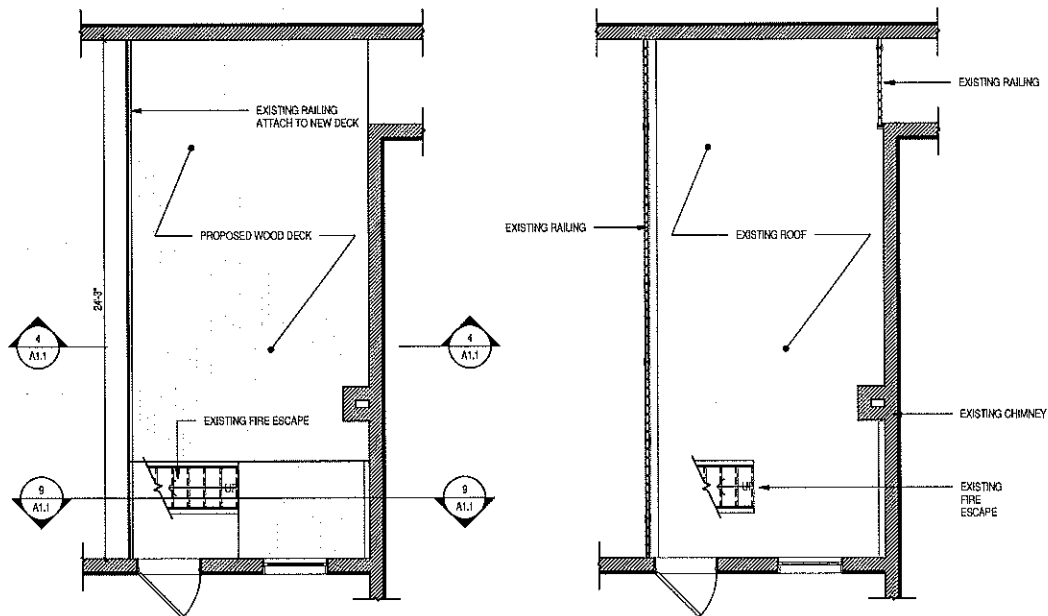
1 PROPOSED ROOF DECK 1/4" = 1'-0"
