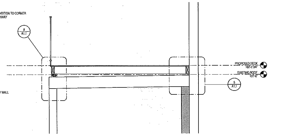
4 PROPOSED SECTION1 1/2" = 1'-0"
