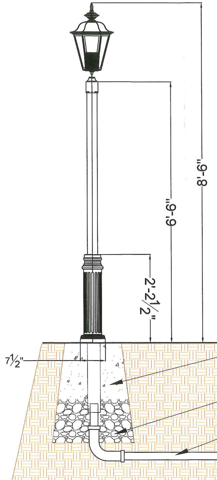
LIGHTING DETAIL- INSTALLATION HERITAGE LIGHT ON FLUTED BASE AND SMOOTH SHAFT, DIRECT-BURIAL POLE
