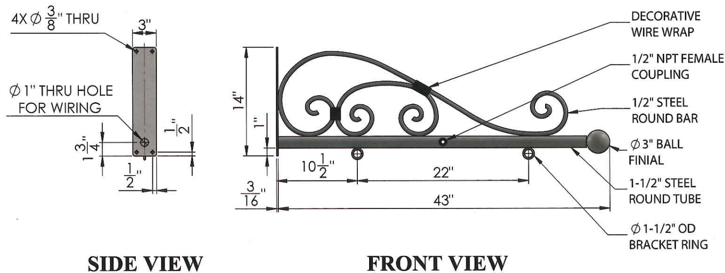
Sign Bracket with External Spot Lighting
